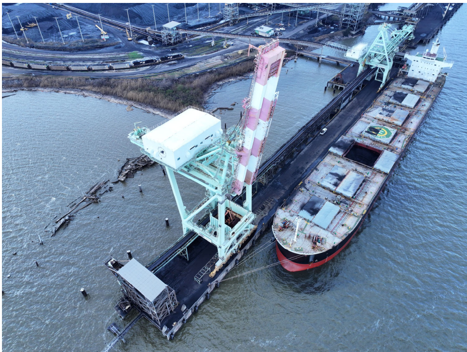
Figure 4: "S" Crane with ship loader on north end of Dock 1
